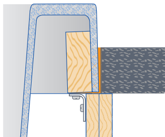
SILGRANIT™ PuraDur™: Module between
